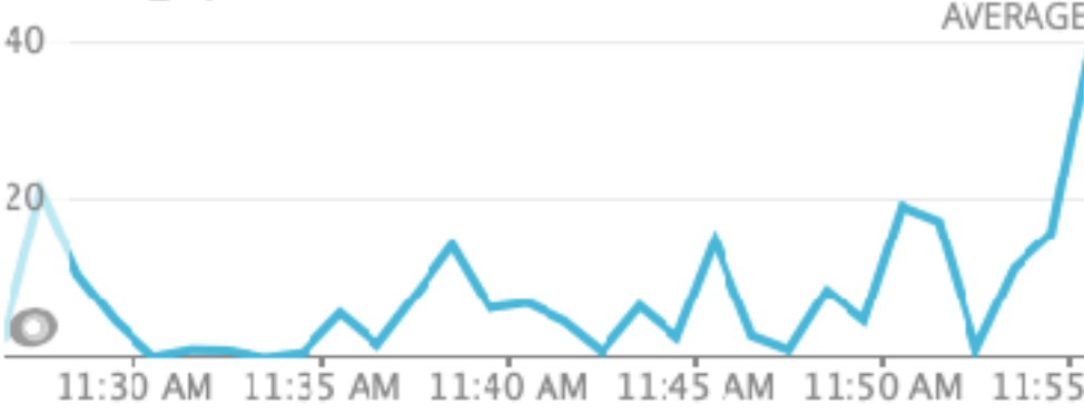
Throughput
