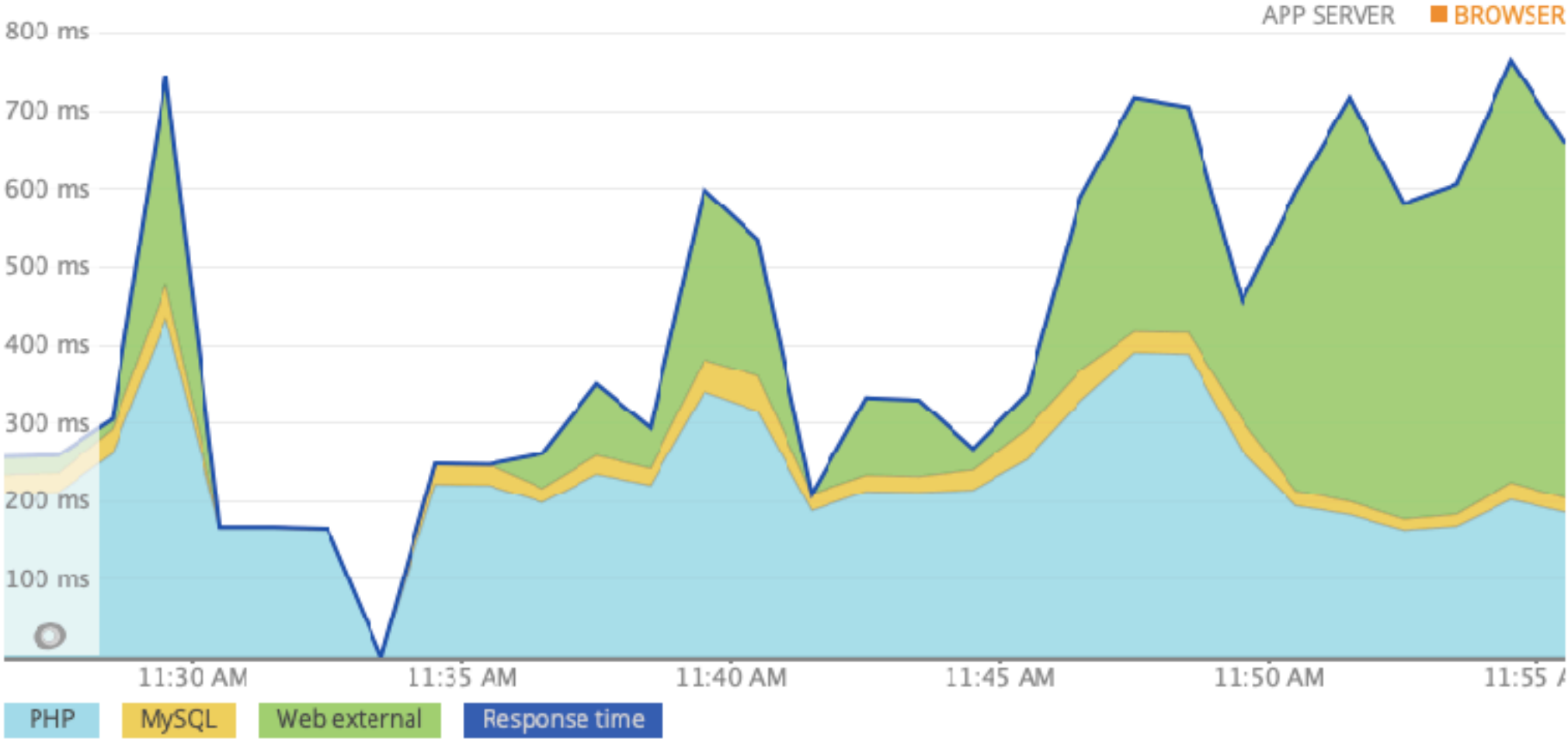
Web transactions time
