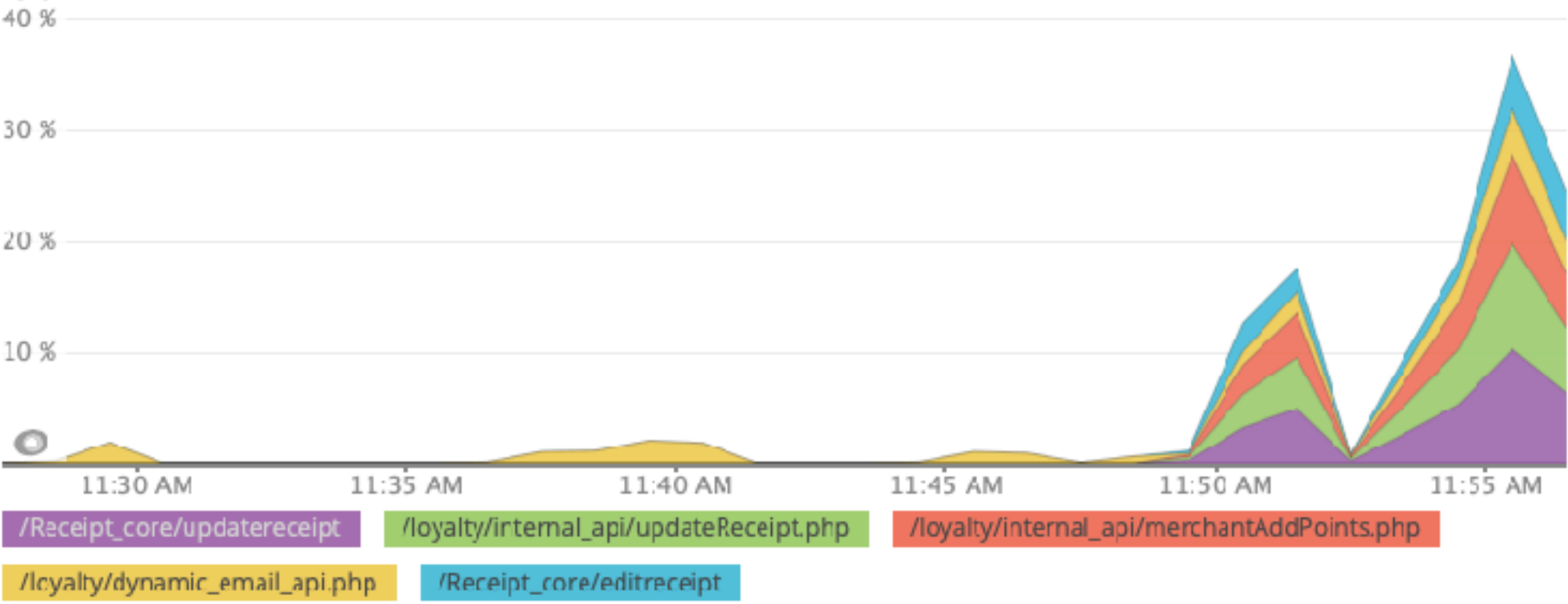
Top 5 web transactions by percent of wall clock time
